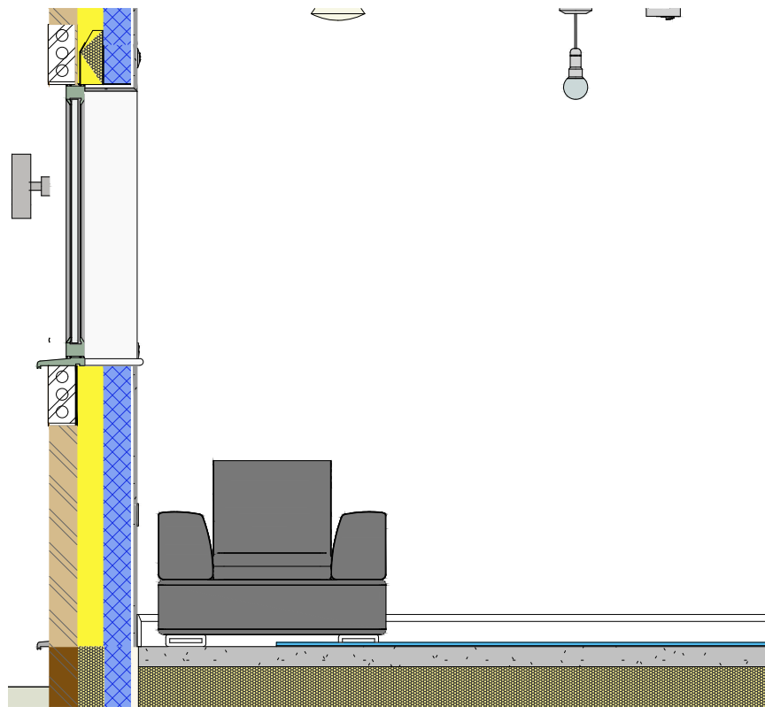
C Kitchen - View C 1 : 25
