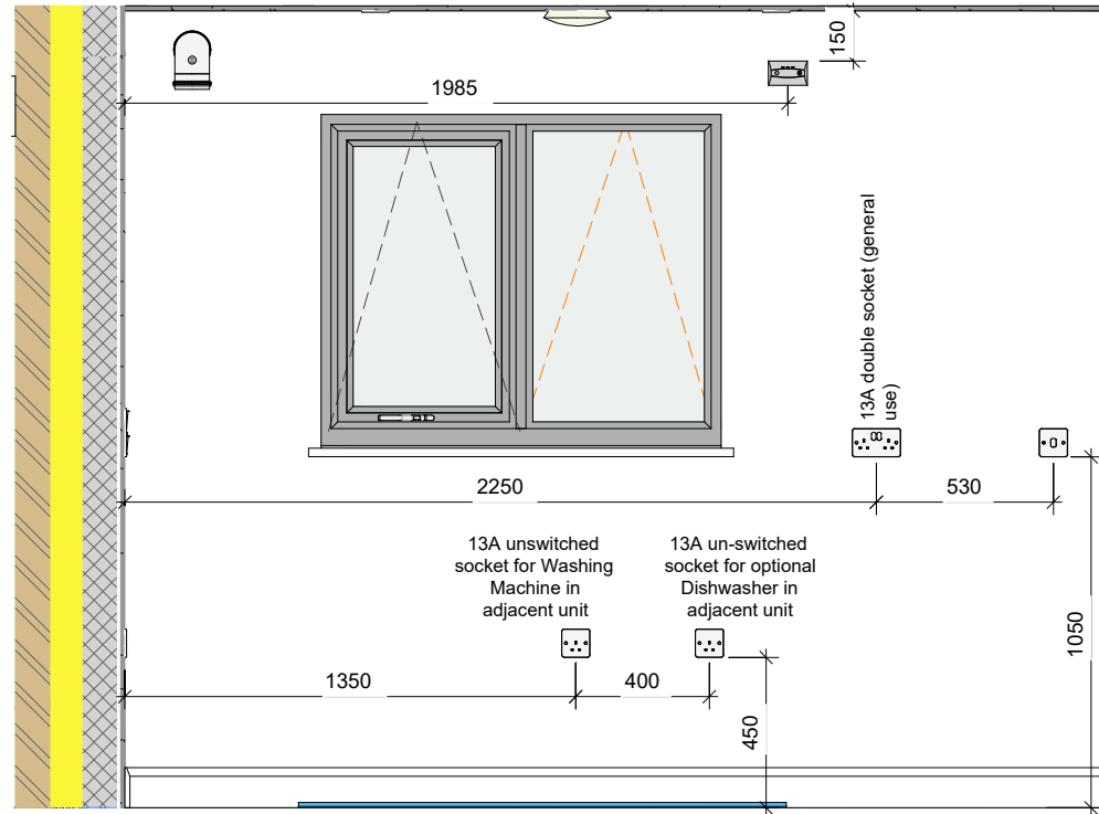
B Kitchen - View B 1 : 25
