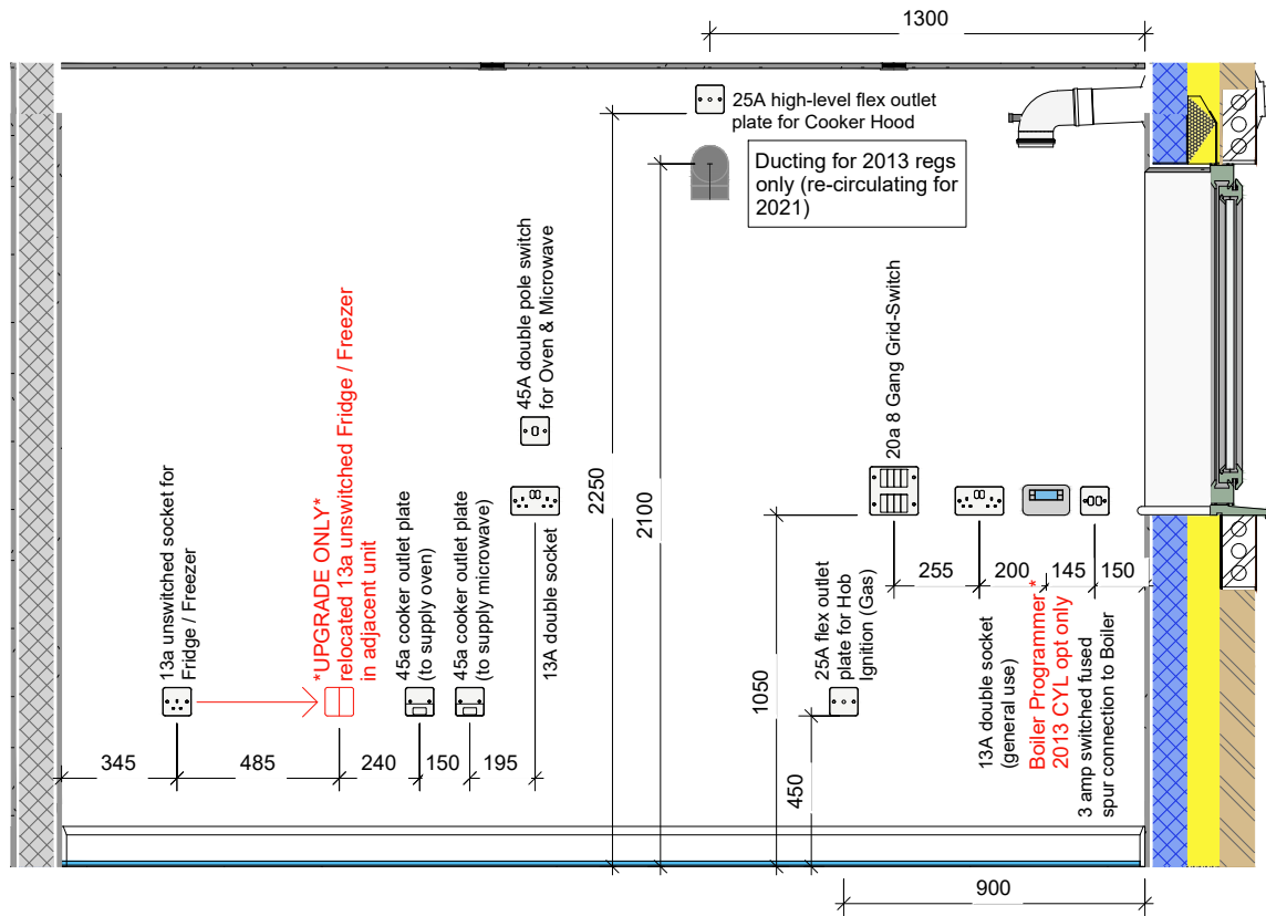
A Kitchen - View B 1 : 25
